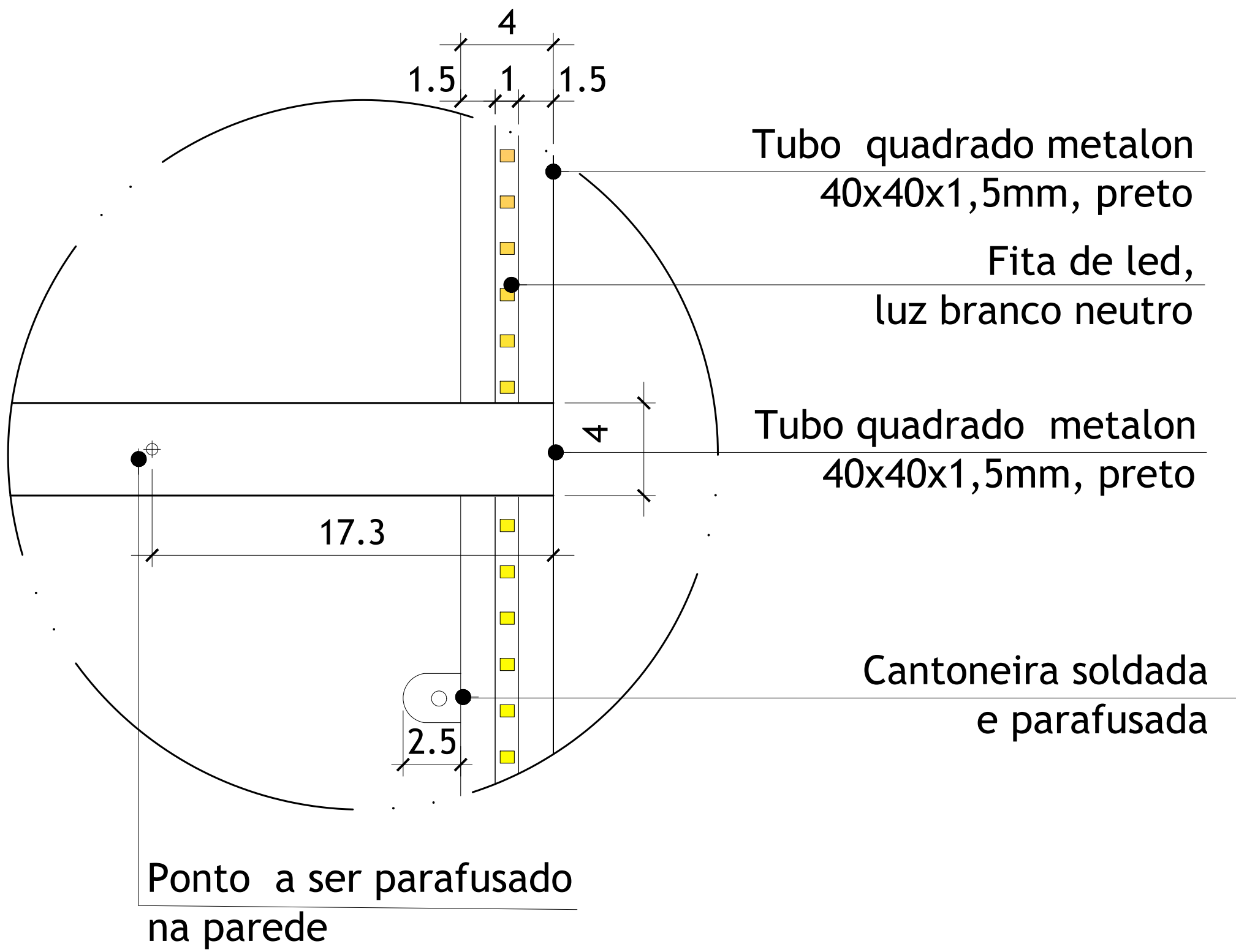
DET 01- FITA DE LED ESCALA 1:2
